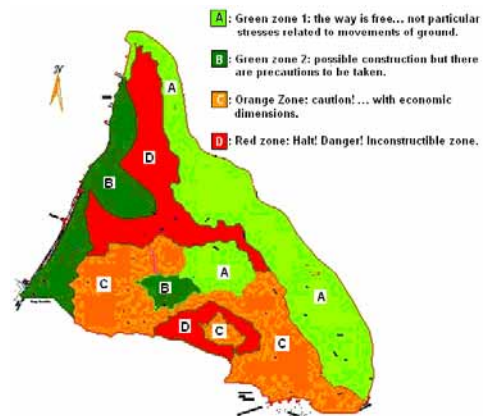
Figure 7. The Risks map of the ZHUN East of Saïda
