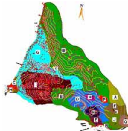
Figure 5: Geotechnical map of ZHUN East of Saïda
