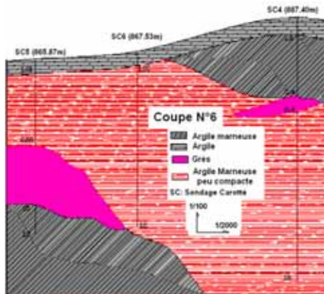
Figure 4: Example geotechnical profile
